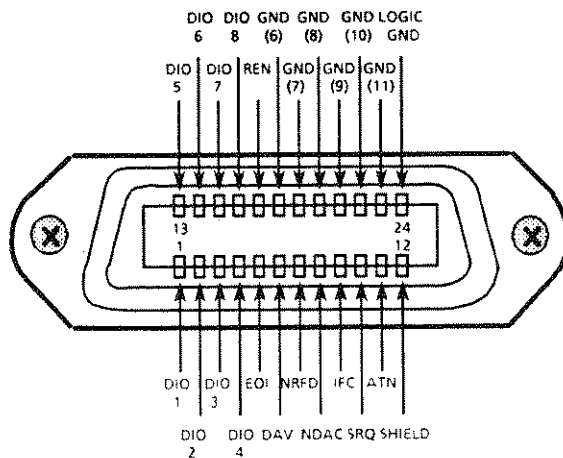
Fig. 2-8 Pin assignment
